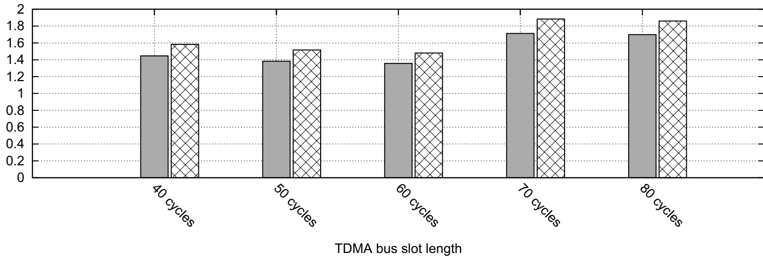
WCET overestimation sensitivity w.r.t bus slot length
