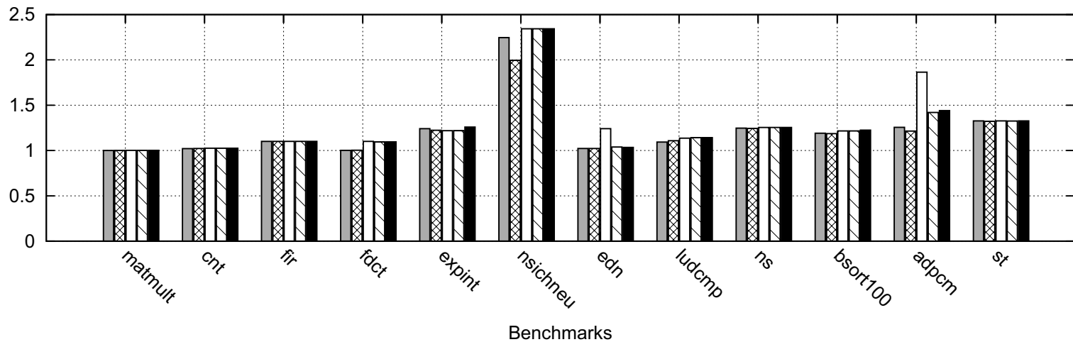
WCET overestimation w.r.t various L2 cache setting
