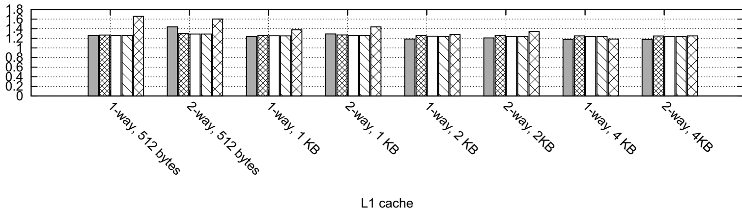
WCET overestimation sensitivity w.r.t L1 cache size
