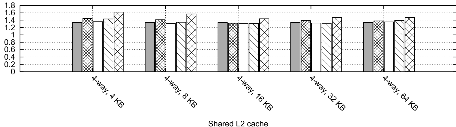
WCET overestimation sensitivity w.r.t L2 cache size
