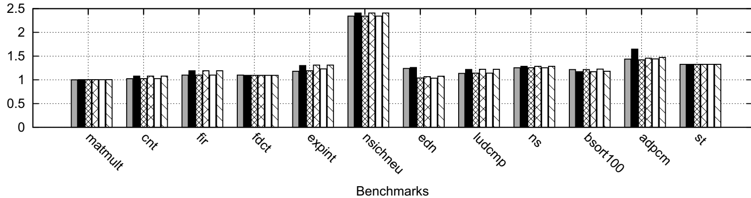
WCET overestimation w.r.t speculation in various L2 cache setting
