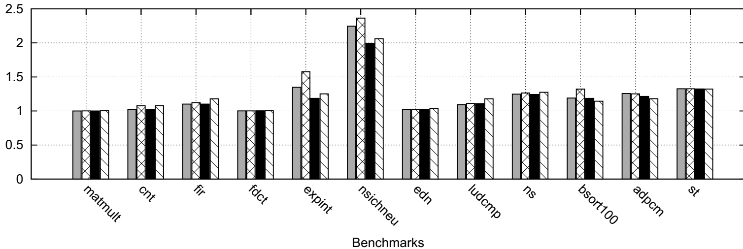
WCET overestimation w.r.t speculation and with only L1 cache
