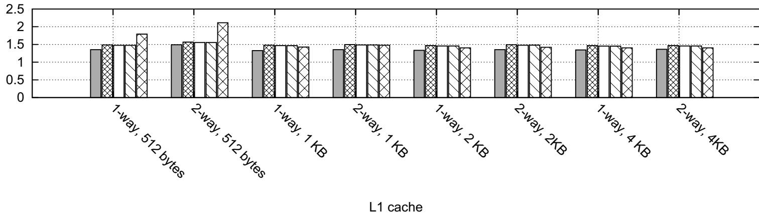
WCET overestimation sensitivity w.r.t speculation and L1 cache size
