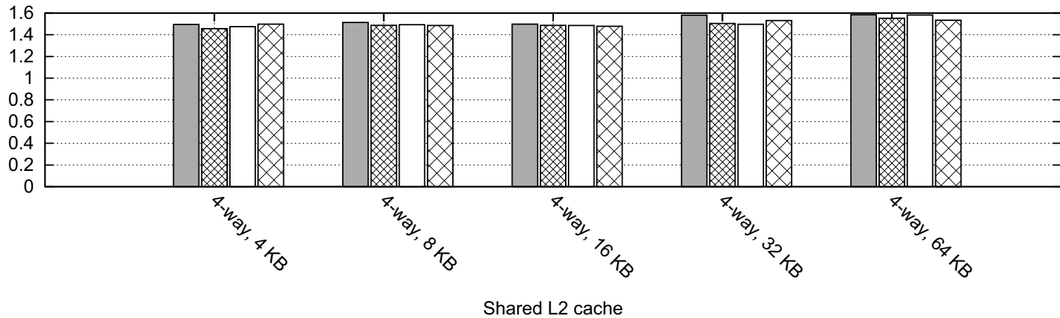
WCET overestimation sensitivity w.r.t speculation and L2 cache size
