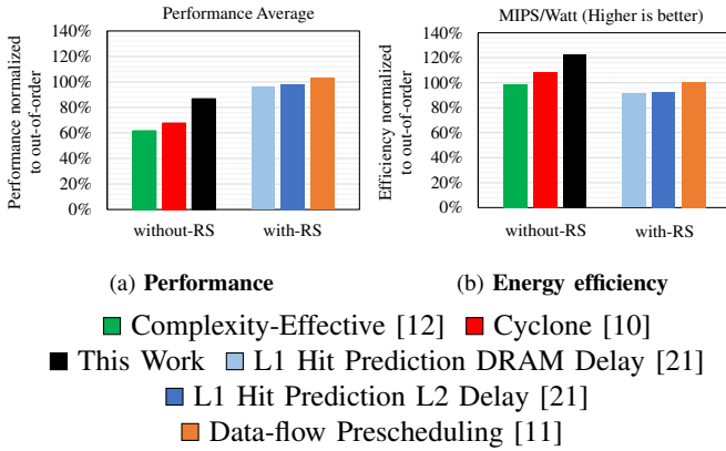
Fig. 5: (a) Performance and (b) Energy efficiency of state-of-the-art issue time prediction processors, normalized to the baseline out-of-order processor.
