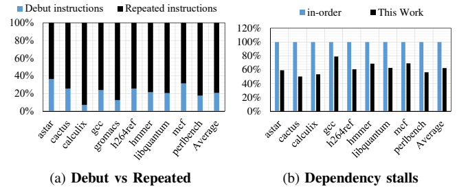
Fig. 7: (a) Cycles spent executing Debut instructions (appear for the first time or miss in the DelayCache) and Repeated instructions (hit in the DelayCache), (b) Cycles the instruction queues are blocked due to unresolved dependencies.
