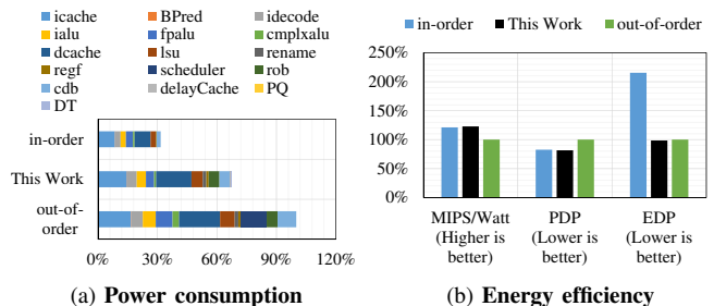
Fig. 4: Normalized to the out-of-order: (a) Power consumption, (b) Efficiency (MIPS/Watt), Power Delay Product (PDP) and Energy Delay Product (EDP).
