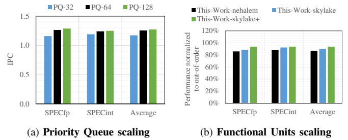
(a) Priority Queue scaling (b) Functional Units scaling
