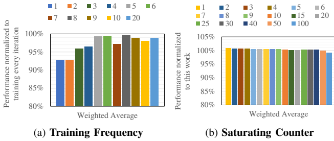
Fig. 9: (a) Train for a number of iterations and use that prediction thereafter (normalized to training every iteration), (b) Use a saturating counter to update the delay every N identical consecutive delays (normalized to This Work). Note that the y-axis starts at 80%.
