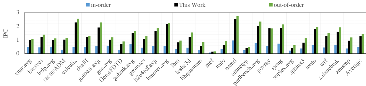
Fig. 3: Performance of the proposed implementation compared to in-order and out-of-order baseline processors. For clarity, we plot average values for applications with multiple inputs ( \langle application\_name \rangle.avg ).
