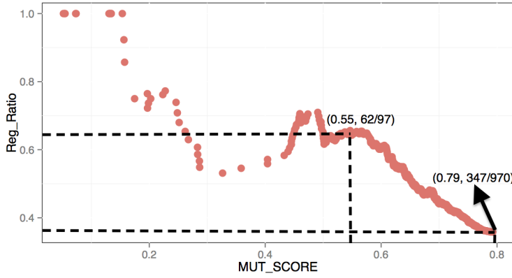
Fig. 3: A scatter plot that illustrates the correlation between the mutation score (the MUT_SCORE axis) and the regression ratio (the Reg_Ratio axis). Coordinate (0.55, 62/97) of the plot describes the following. First, among test-suites with which repairs are successfully generated, there are 97 test-suites whose mutation scores are not greater than 0.55. Second, out of these 97 cases, a regression is detected in 62 cases. Similarly, coordinate (0.79, 347/970) describes that there are 970 test-suites whose mutation scores are not greater than 0.79, and a regression is detected in 347 cases.
