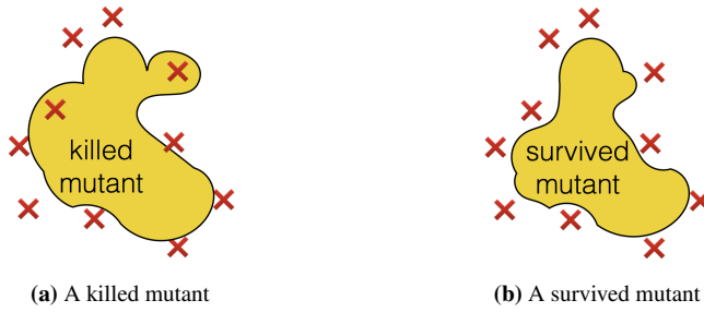
Fig. 1: The cross marks represent the tests in a test-suite. Crossing over a cross mark means that the mutant fails the corresponding test.
