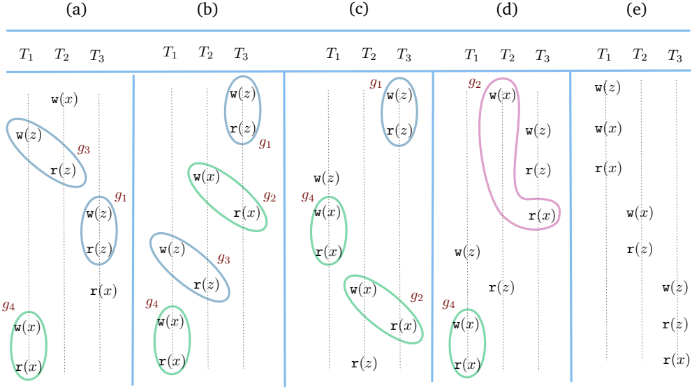
Fig. 3. Examples 4.3, 6.1, and 6.2.
