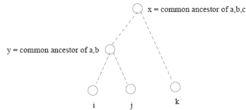
Figure 8.4: Ultrametric Tree
