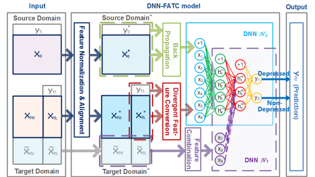
Figure 1: An illustration of our framework.
